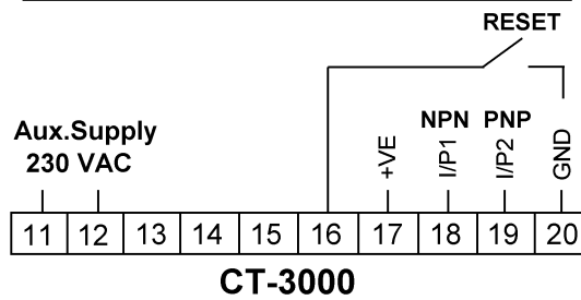
Micro Switch: Micro switch Connection to 18 & 20
