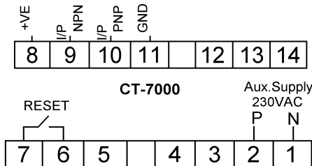
Micro S/W: M/S connection 9 & 11
