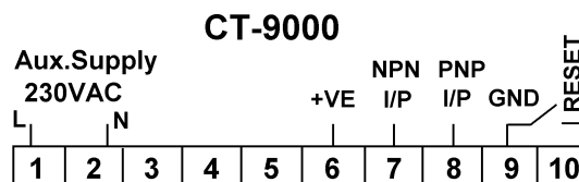
Micro Switch: Micro Switch connection to 7 & 9
